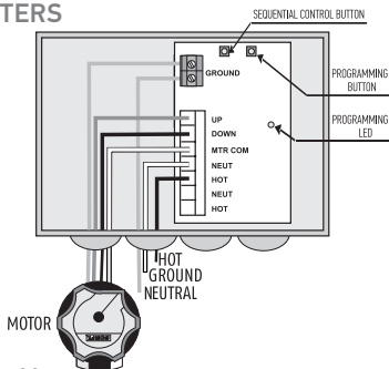
NEW transmitter
