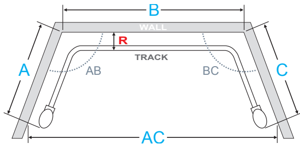
STYLE 3 MEASUREMENT
